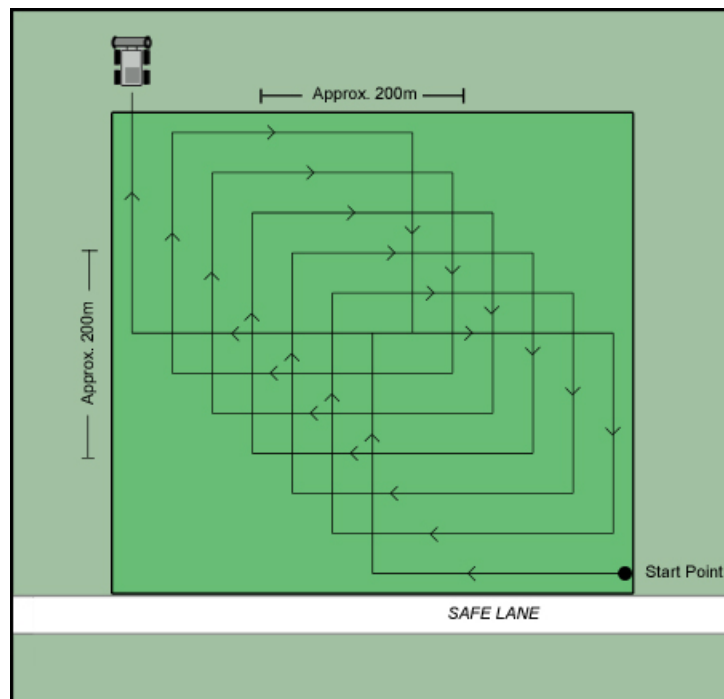
Fig. 1: Section of a piece of land in a suspect area (approx. 200m x 200m). 1 st phase of rolling in concentric box pattern in area where mines are not expected. Pattern is optional but this technique has been proven effective.
